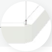
Suspension points with 2 or 3 modules joints
